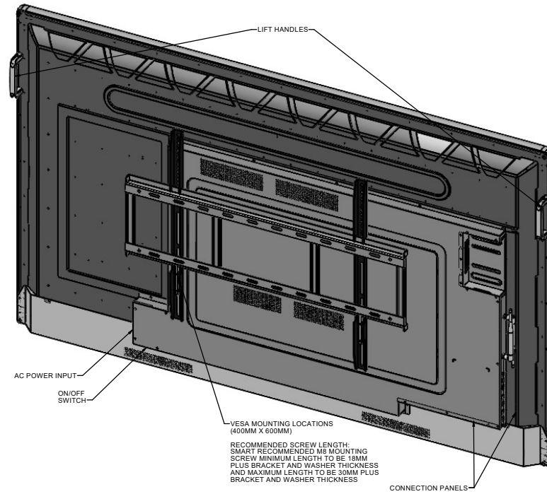
REAR TRIMETRIC VIEW
